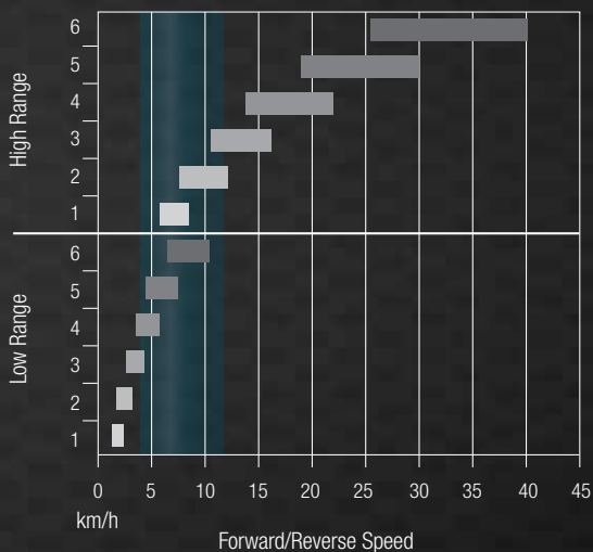
Dyna Synchronshift 12x12 Transmission
